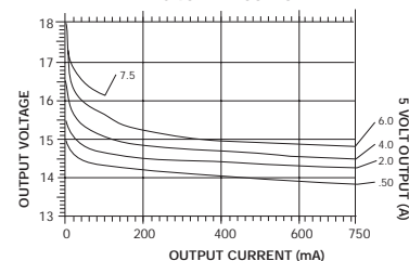
Auxiliary Load Regulation NFC40-XXT05-15-M
