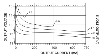
Auxiliary Load Regulation NFC40-XXT05-15-M
